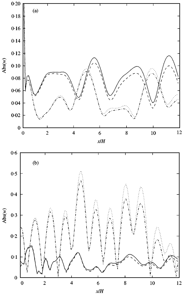
Figure 7. Dimensionless displacements on the upper surface of a [C90/G + 45/G - 45]_s plate subjected to a Gaussian beam with shape factor b = 0.01 . (a) The Gaussian beam frequency is \bar{\omega} = 3.14 . (b) The Gaussian beam frequency is \bar{\omega} = 6.28 . — Fluid-plate-free, p = 0.0 ; --- Fluid-plate-free, p = 0.01 ; .... Fluid-plate-fluid, p = 0.0 ; - · - · - Fluid-plate-fluid, p = 0.01 .
