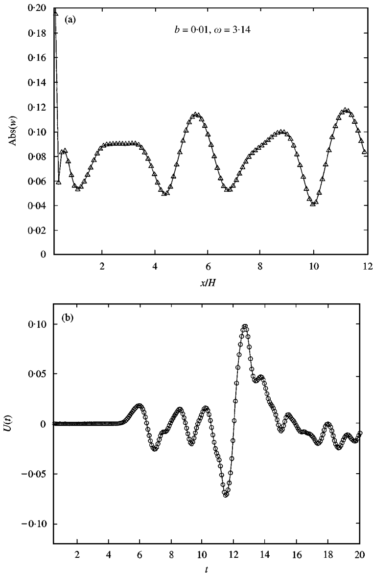
Figure 3. Dimensionless displacement on the upper surface of a [C90/G + 45/G - 45]_s plate. (a) Comparison in frequency domain, — Liu et al. [7]; \triangle Present analysis. (b) Comparison in time domain, — Liu et al. [7]; \circ Present analysis.
